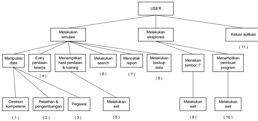
Gambar 4. Task Analysis Model
