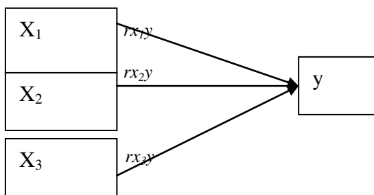
Gambar 3.1 Variabel Penelitian
