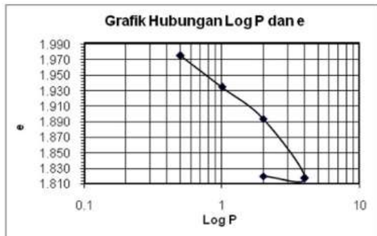
Gambar 2.22 Plot e – log P
