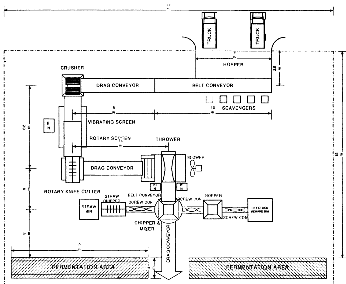
Figure 2. Plant Layout
