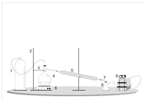
Gambar 1. Rangkaian alat polimerisasi (1) Tabung gas N 2 , (4) labu alas bulat, (5) kondensor, (6) hot plate stirrer, (8) erlenmeyer, (9) pompa vacum
