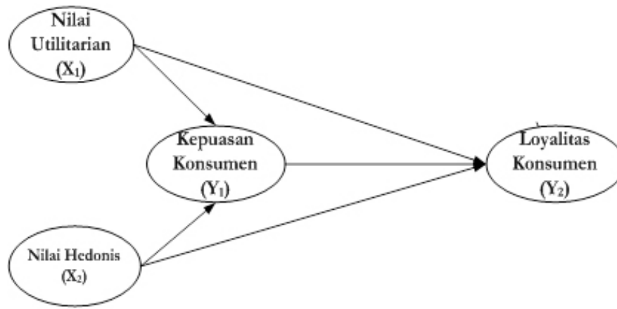
Gambar 1. Model struktural variabel penelitian
