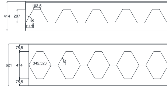
Gambar 3 Potongan Memanjang Castellated Beam
