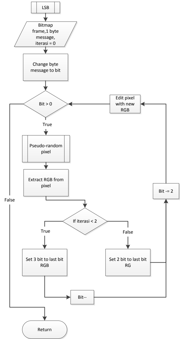
Figure 4. LSB Flowchart
