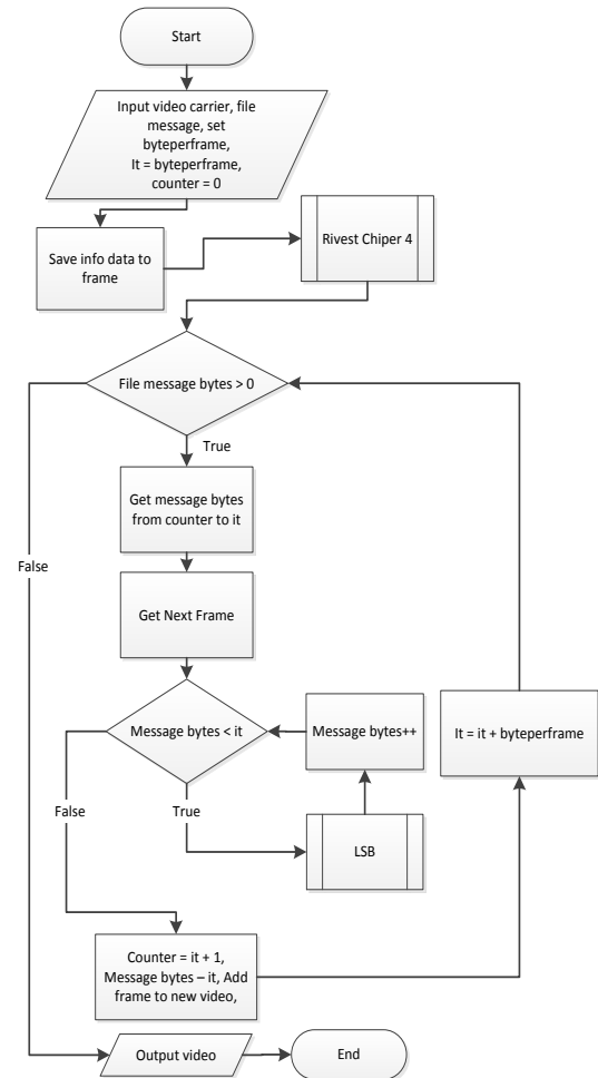
Figure 2. Steganography Flowchart
