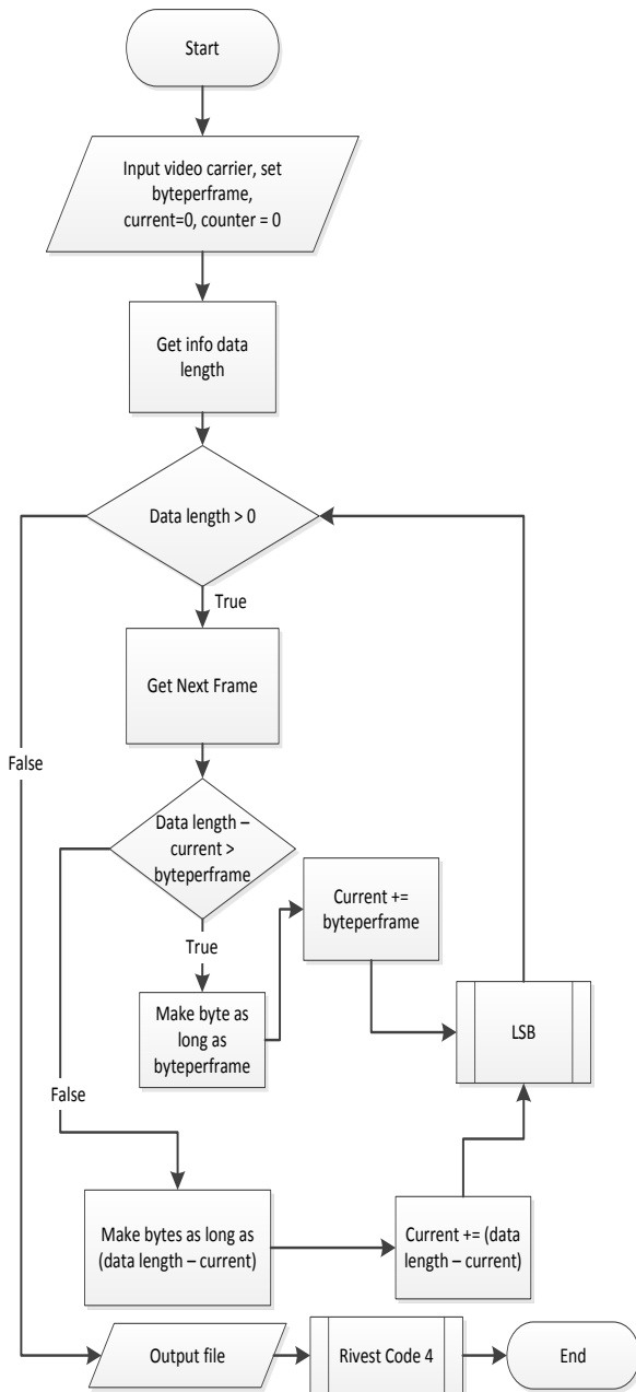
Figure 5. Extracting Flowchart
