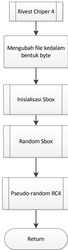
Figure 3. Rivest Code 4 Flowchart
