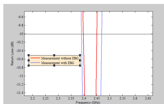
Figure 8. Bandwidth Comparison of measured microstrip antenna with and without EBG
