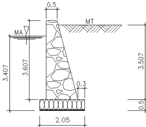
Gambar 6. Dinding Penahan Tanah Sungai Sringin
