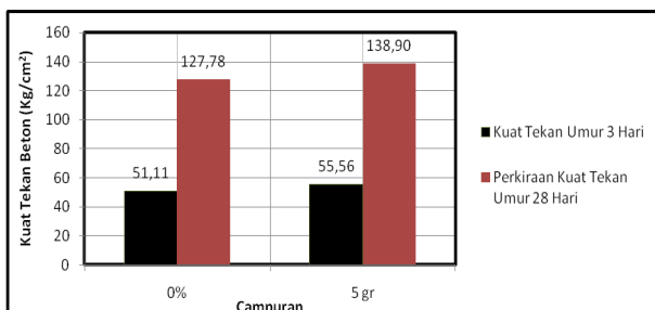
Gambar Diagram Kuat Tekan Beton
