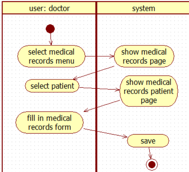
Gambar 6. Activity Diagram Rekam Medis
