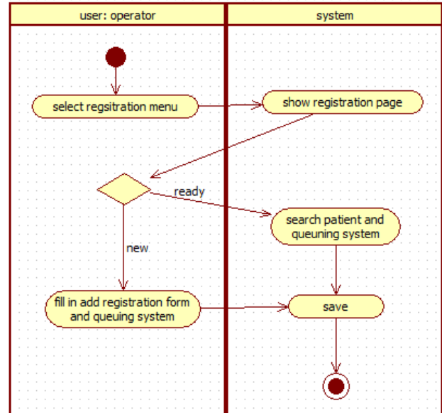
Gambar 4. Activity Diagram Registrasi Pasien
