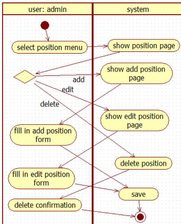
Gambar 7. Activity Diagram Rekam Medis
