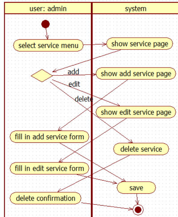
Gambar 8. Activity Diagram Rekam Medis
