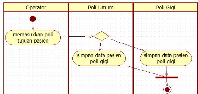
Gambar 5. Activity Diagram Poli
