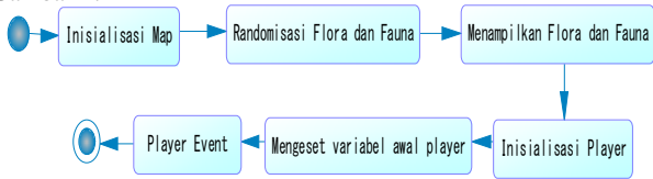
Gambar 4 Flowchart Game Labirin
