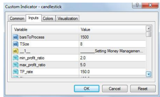
Gambar 6 Setting Awal
