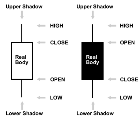
Gambar 1 Candlestick
