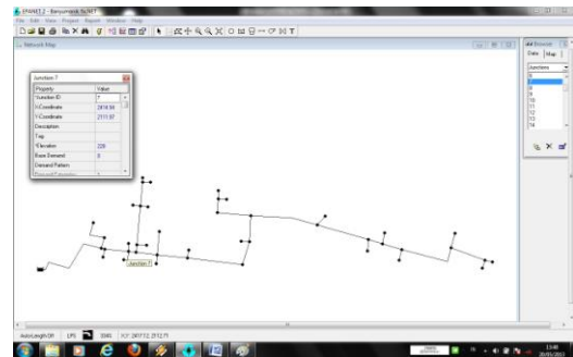
Gambar 4.2. Pengisian Junction
