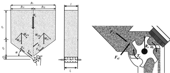
Gambar 3. Analisis pendugaan torsi rotor edge-cell
