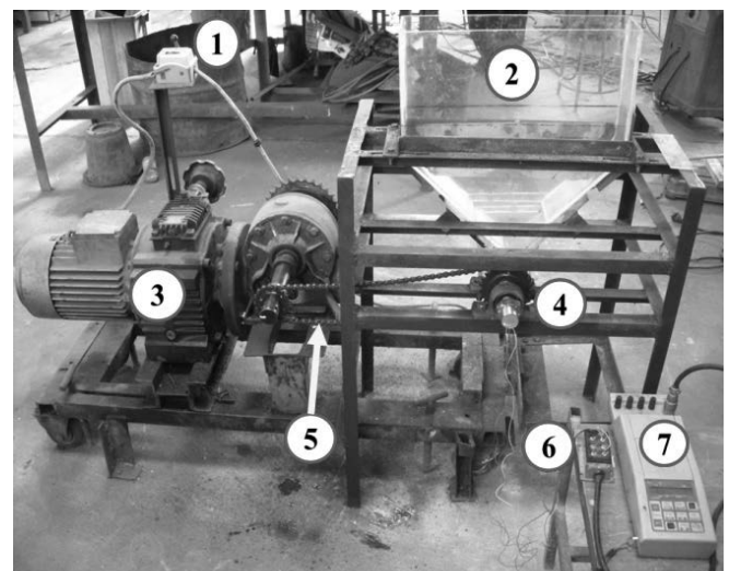
Keterangan: 1. Saklar 2. Hopper 3. Motor AC variable speed 4. Poros penjajah dan slip ring 5. Rantai 6. Bridge box 7. Handy strain meter
