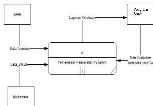
Gambar 2. Context Diagram
