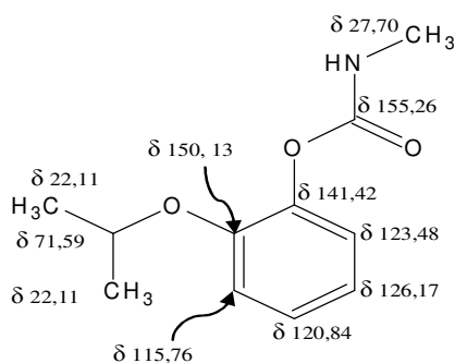
Gambar 3 Nilai pergeseran kimia ( ^{13}\text{C} )
