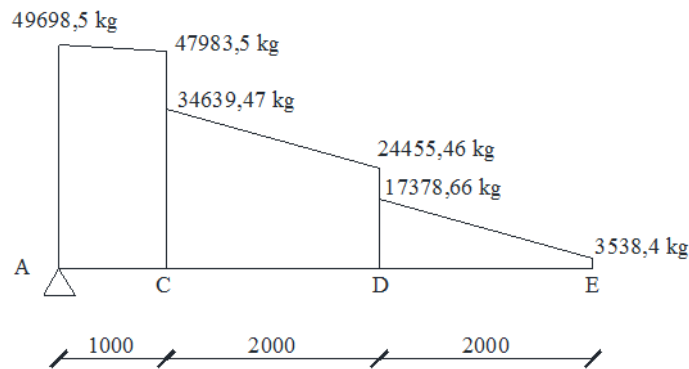
Gambar 7. Diagram Gaya Lintang
