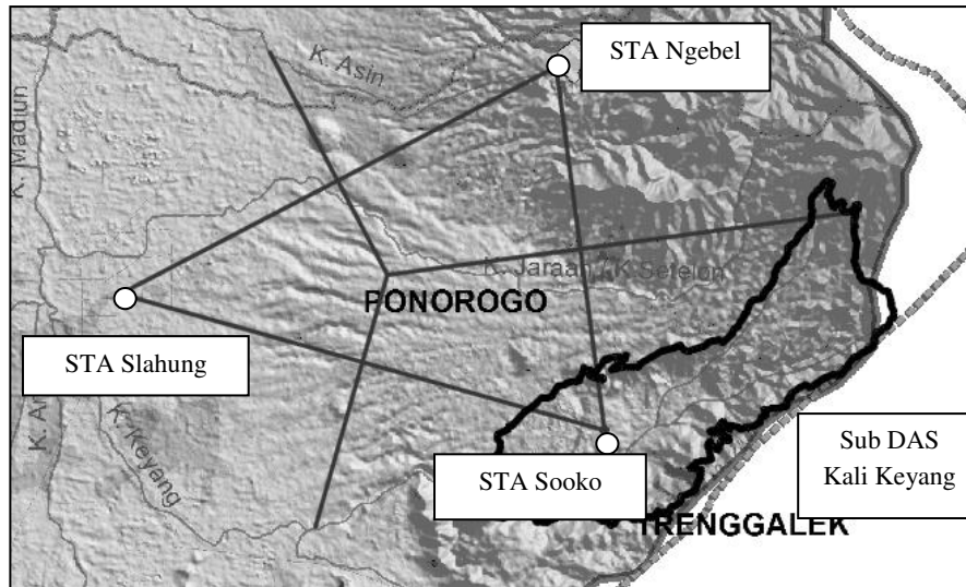
Gambar 6. Poligon Thiessen Sub DAS Kali Keyang
