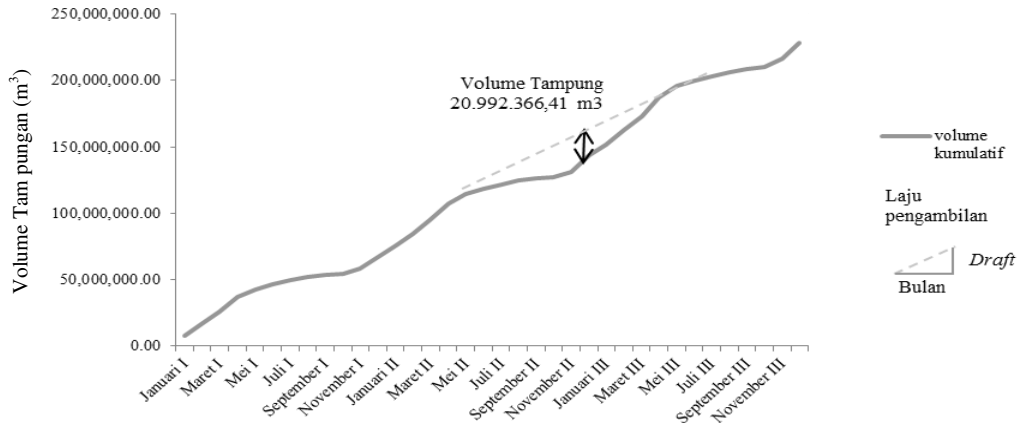
Gambar 7. Mass curve kumulatif inflow – outflow
