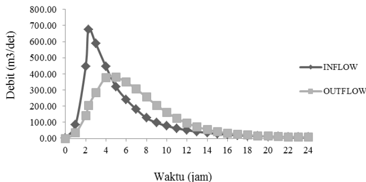
Gambar 8. Grafik Hidrograf Q 1000th Inflow – Outflow Pelimpah
