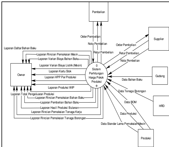
Gambar 1. DFD Context Diagram
