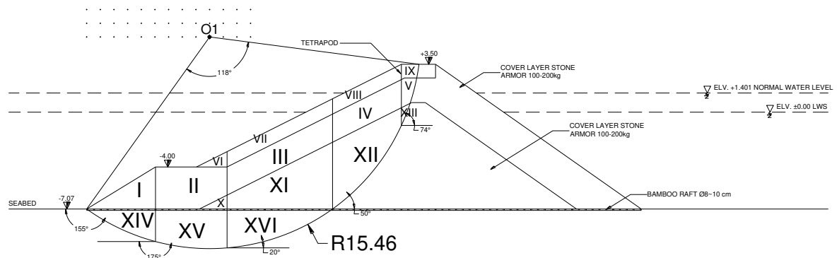
Gambar 8. Permodelan Lereng Breakwater Sta.00+350 R = 15.46 m
