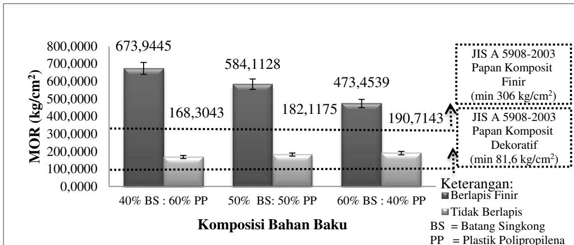
Gambar 6. Nilai Rerata Modulus Patah ( \Delta MOR) Papan Komposit Berdasarkan Pelapisan dan Komposisi Bahan Baku ( The Average Modulus of Rupture of Composite Board Based on Coating and Composition of Raw Material )
