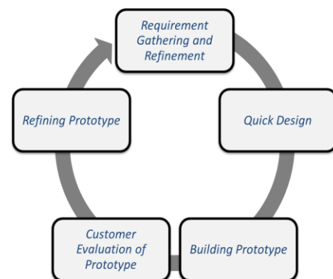
Gambar 3. Metode Prototype
