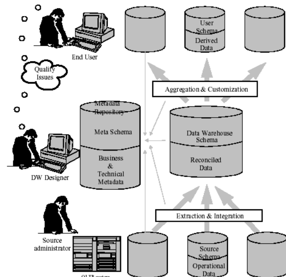
Figure 2. Architecture for a Data Warehouse
