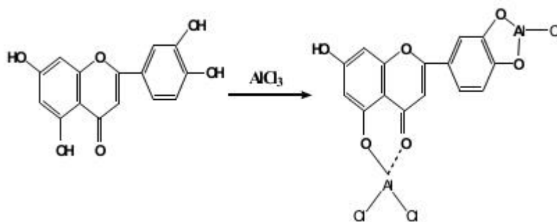
Figure 3. Complex-forming reaction between flavonoid and aluminum
