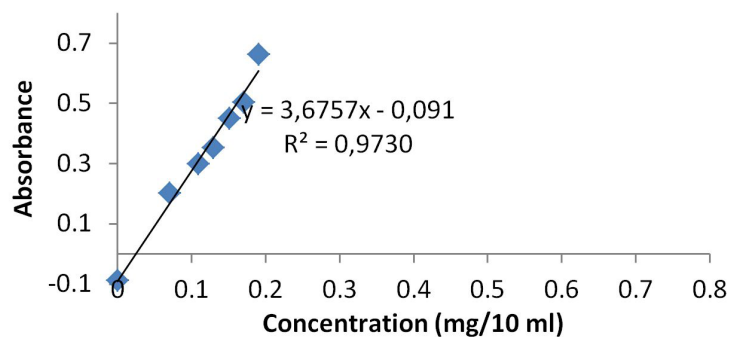
Figure 2. Graph of Correlation between Concentration and Absorbance of Quercetin Solution
