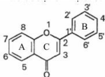
Figure 1. Flavonoid structure 11
