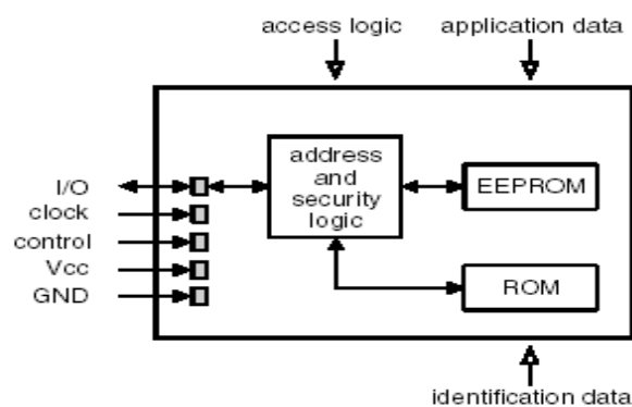
Gambar 2.1 Memory Card
