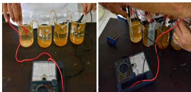
Figure 4 Process of testing electric conductivity of acid mine drainage.
