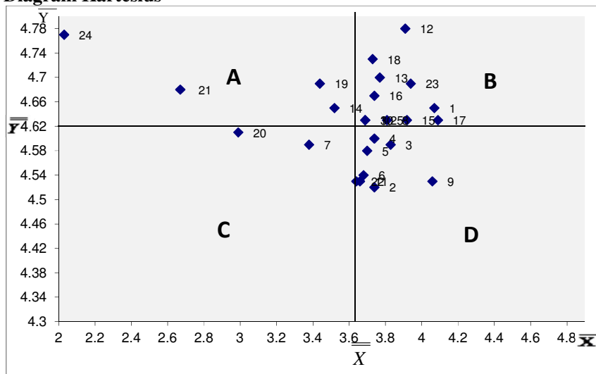
Diagram Kartesius
