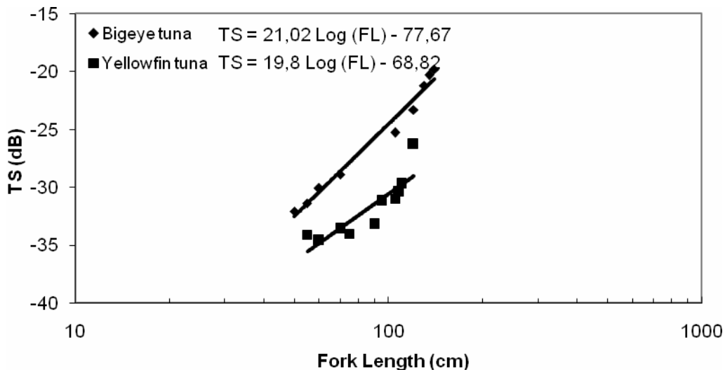
Figure 2. Variation of target strength with tuna fork length (cm) for bigeye and yellowfin tuna. Solid line is the best fit equation TS = a \log FL + b of experimental data. x-axis is a logarithmic scale.
