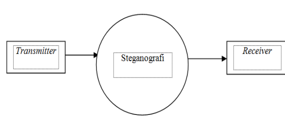
Gambar 1. DFD Level 0
