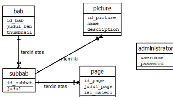
Gambar 3 Entity Relationship Diagram Aplikasi Web Administrator
