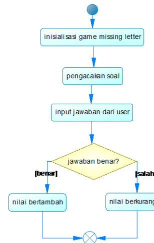
Gambar 3. Flowchart Game Find Missing Letter.
