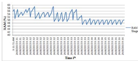
Figure 9. The memory usage of the purposed method.
