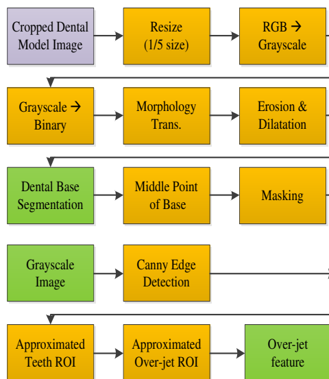
Figure 7. General flowchart for over-jet feature extraction.
