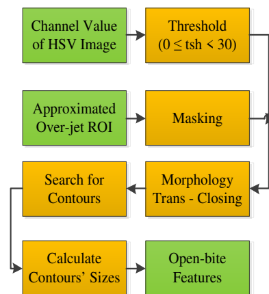
Figure 9. General flowchart for open-bite feature extraction.
