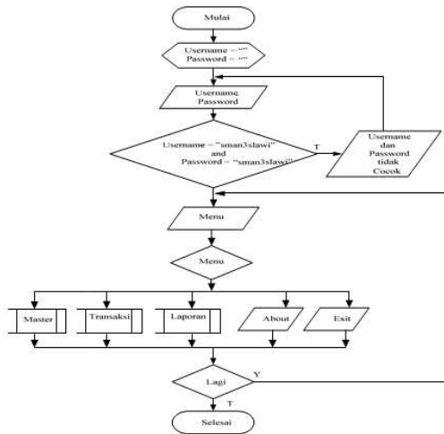
Gambar 1. Flowcart login admin
