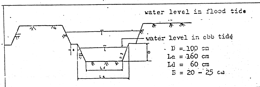
Figure 5. Design examples of the improvement tertiary canals of the TDB
