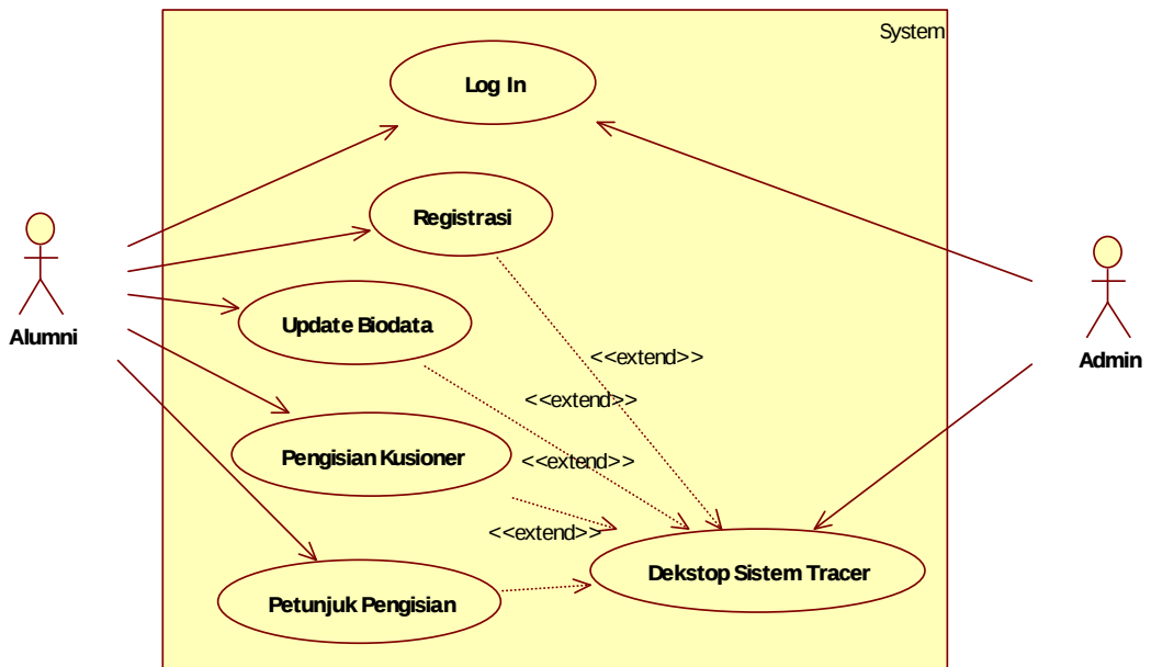
Gambar 3. Use case System
