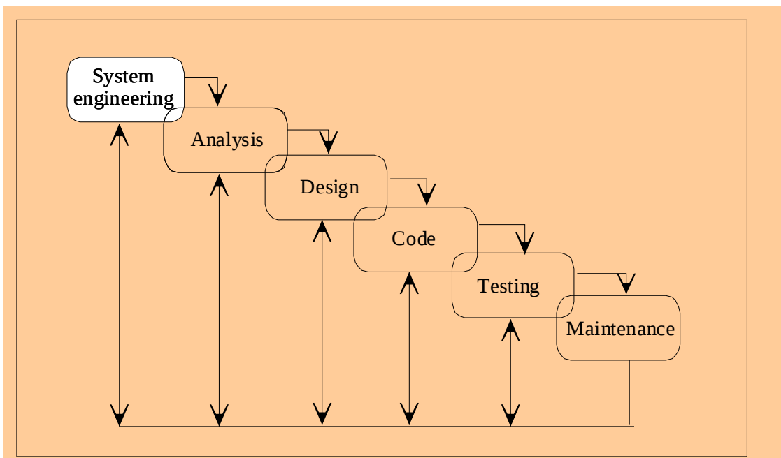
Gambar 1 Paradigma Waterfall
