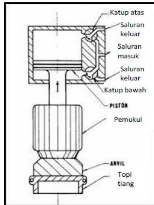
Gambar 3- Double acting power driven hammer
