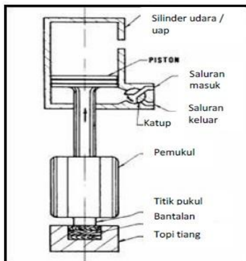
Gambar2- Single acting power driven hammer
