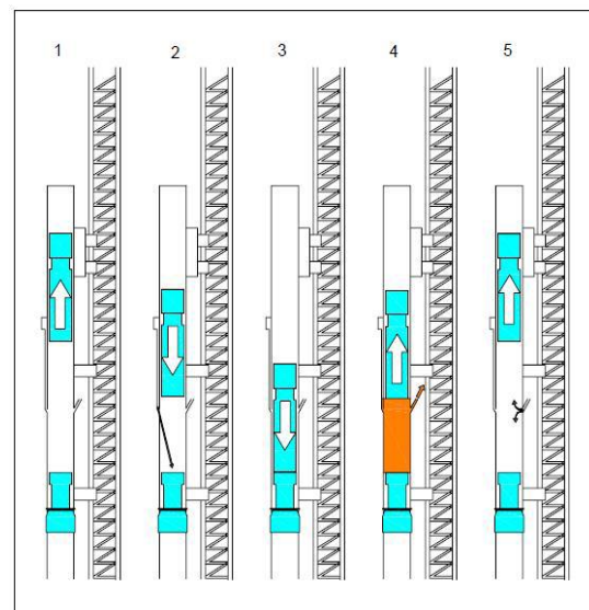
Gambar 4.Mekanisme kerja diesel power driven hammer.
